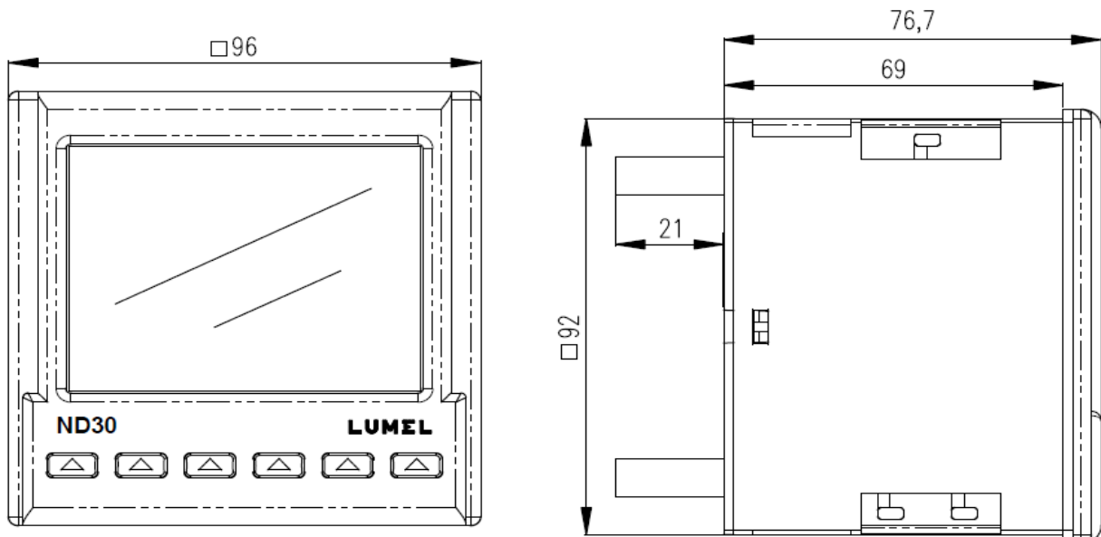
Fig. 3. Overall dimensions of the ND30 meter
