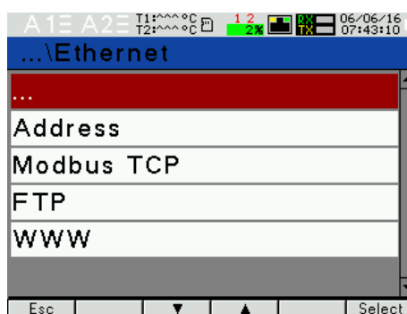
Fig.22. Screens of Ethernet mode
